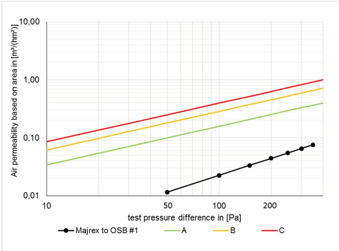
Fig. 12: Series of measurements for the sample "SIGA Majrex to OSB panel #1". The certificate classes A to C according to the PHI are entered in addition.
