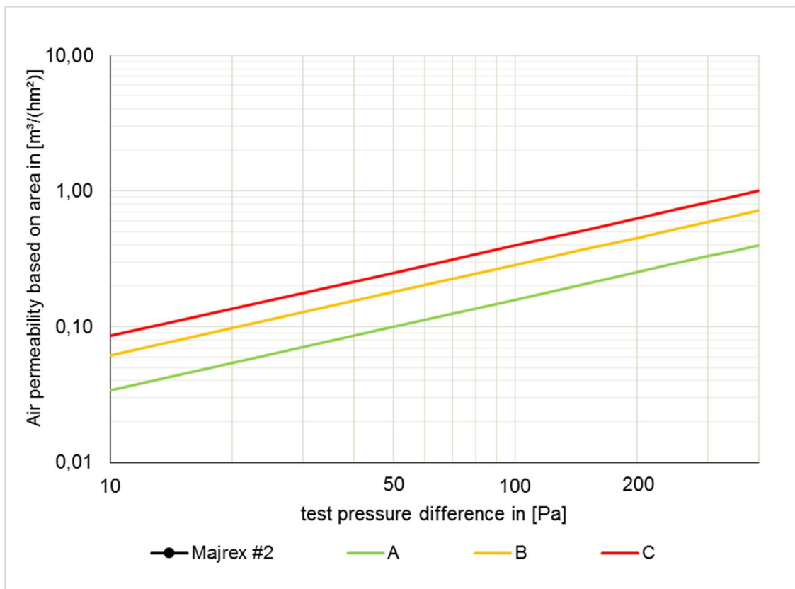
Fig. 7: Series of measurements for the sample "SIGA Majrex 2" (membrane on its own). The certificate classes A to C according to the PHI are entered in addition.
