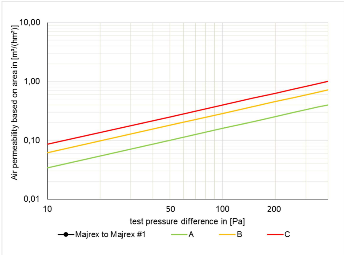
Fig. 9: Series of measurements for the sample "SIGA Majrex to SIGA Majrex #1". The certificate classes A to C according to the PHI are entered in addition
