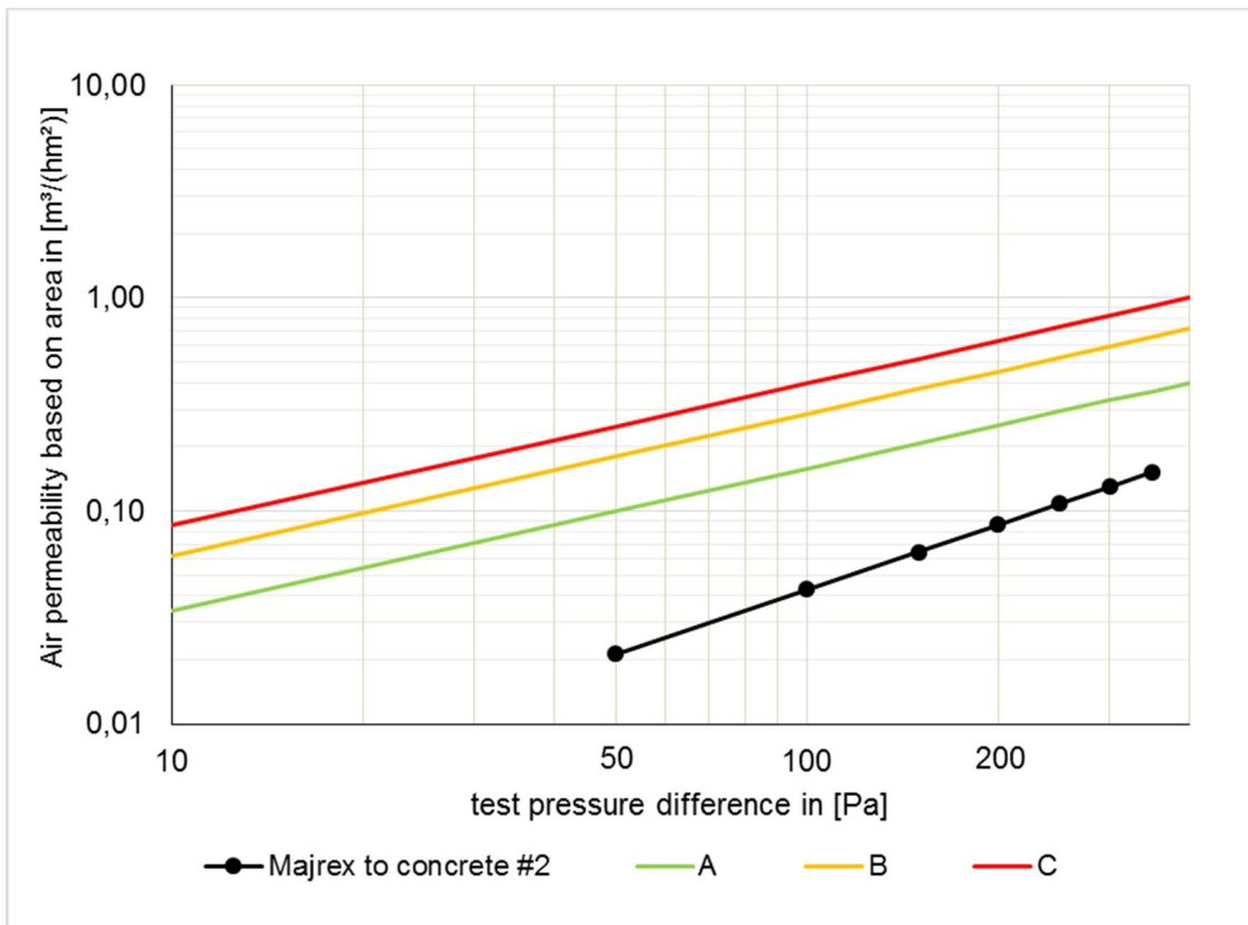
Fig. 16: Series of measurements for the sample "SIGA Majrex to concrete slab #2". The certificate classes A to C according to the PHI are entered in addition.
