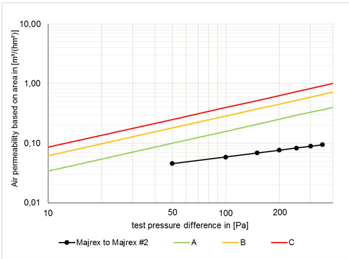
Fig. 10: Series of measurements for the sample "SIGA Majrex to SIGA Majrex #2". The certificate classes A to C according to the PHI are entered in addition.
