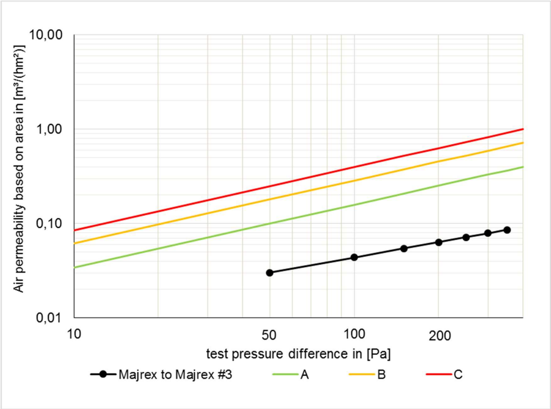
Fig. 11: Series of measurements for the sample "SIGA Majrex to SIGA Majrex #3". The certificate classes A to C according to the PHI are entered in addition.
