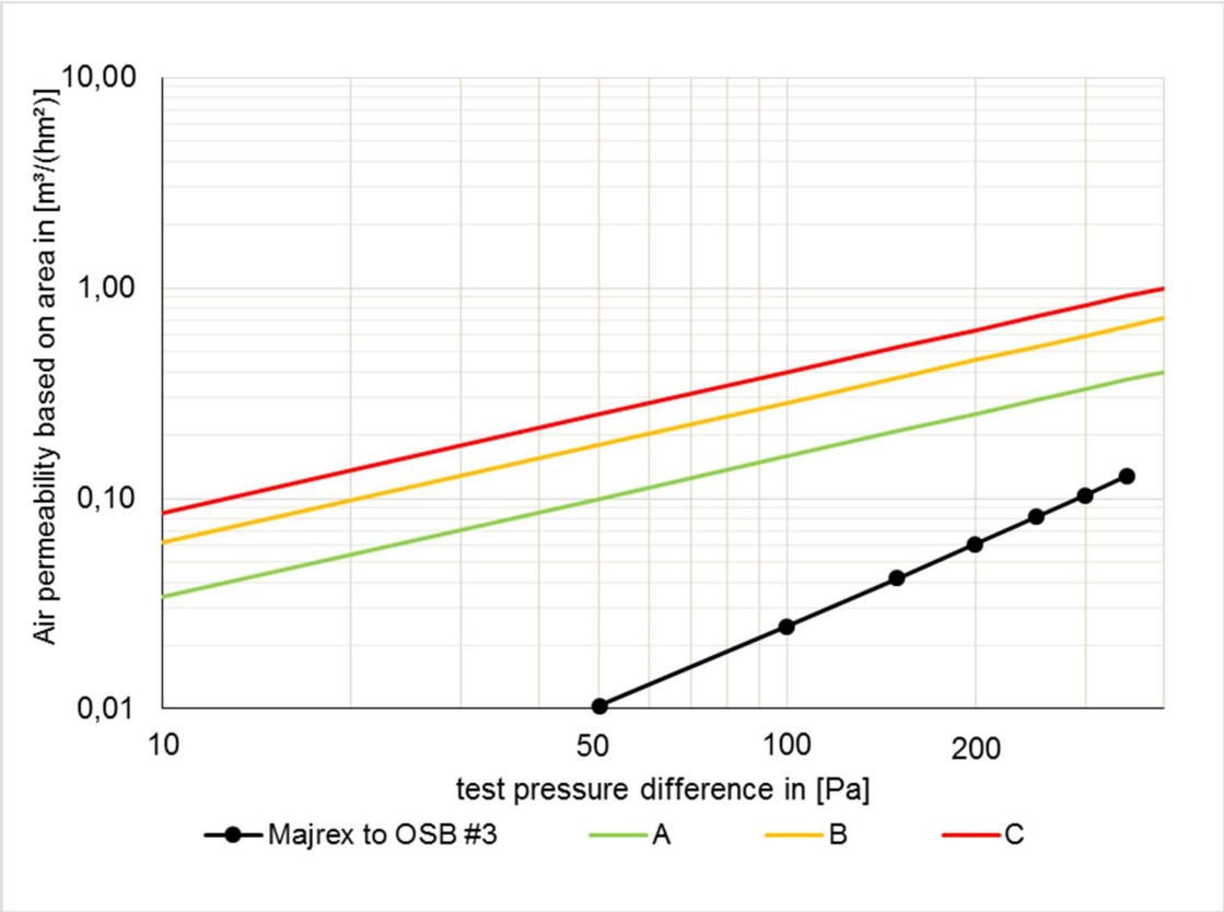
Fig. 14: Series of measurements for the sample "SIGA Majrex to OSB panel #3". The certificate classes A to C according to the PHI are entered in addition.
