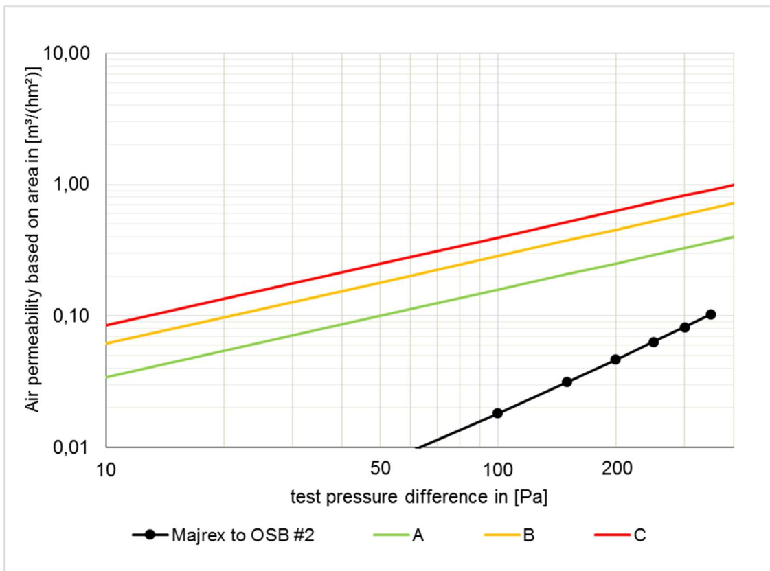
Fig. 13: Series of measurements for the sample "SIGA Majrex to OSB panel #2". The certificate classes A to C according to the PHI are entered in addition.
