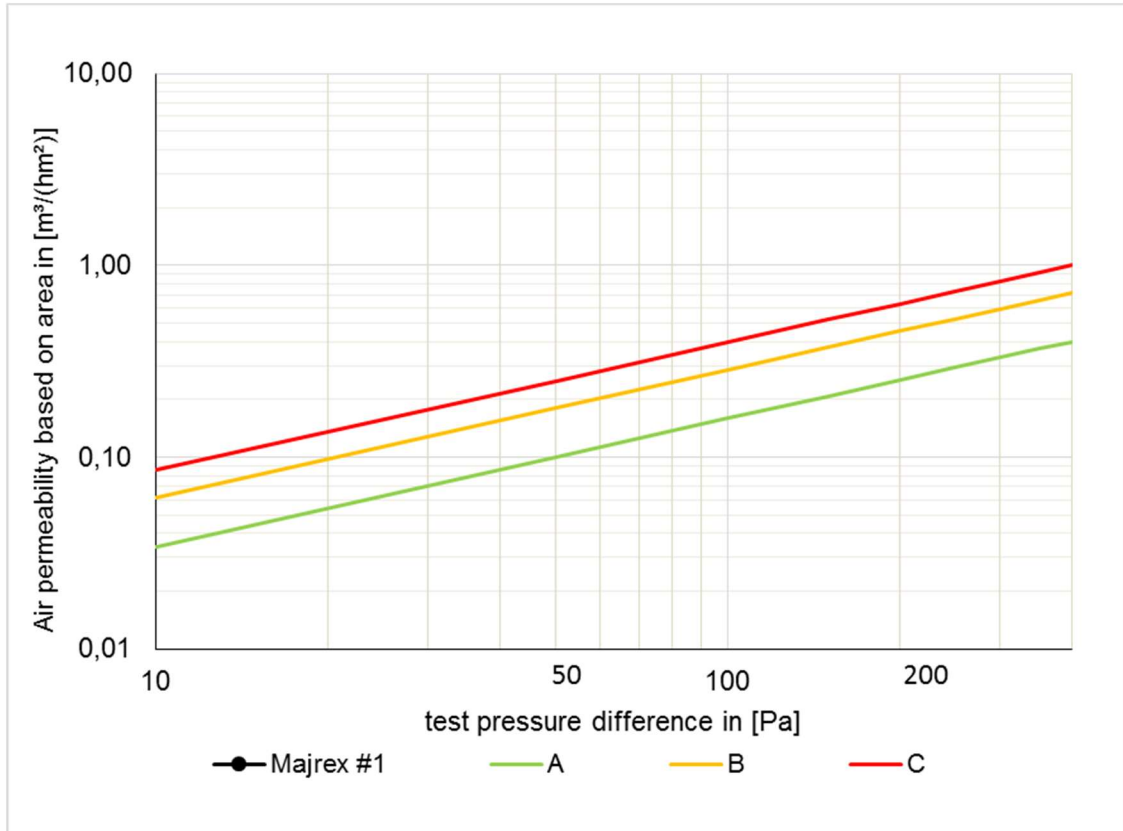
Fig. 6: Series of measurements for the sample "SIGA Majrex 1" (membrane on its own). The certificate classes A to C according to the PHI are entered in addition.
