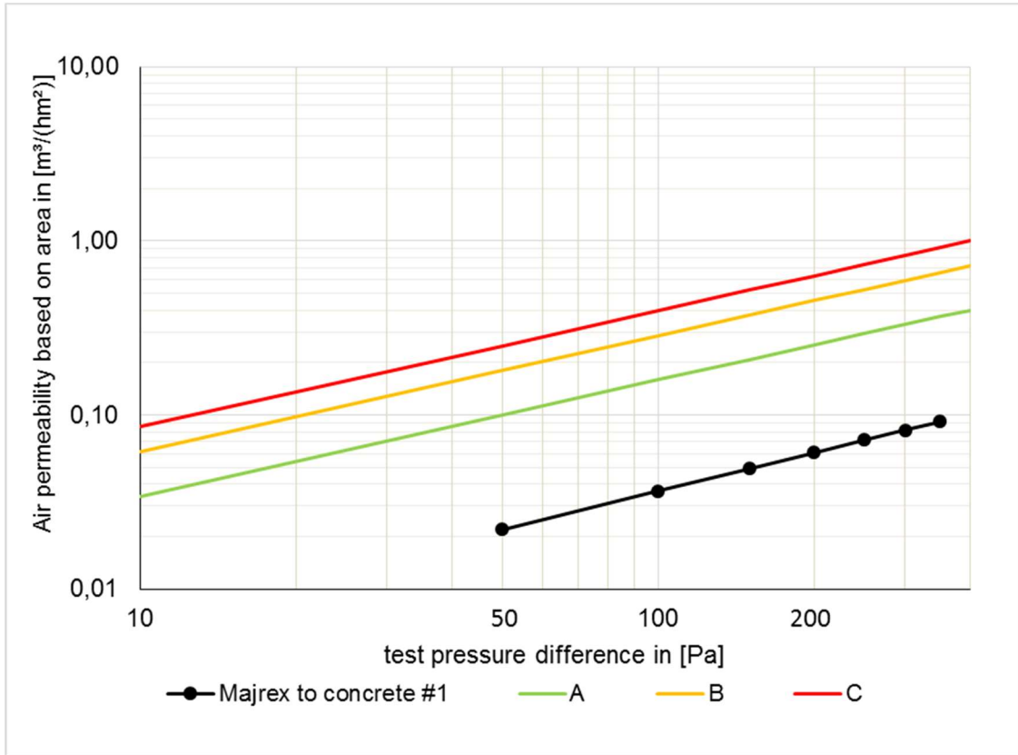
Fig. 15: Series of measurements for the sample "SIGA Majrex to concrete slab #1". The certificate classes A to C according to the PHI are entered in addition.
