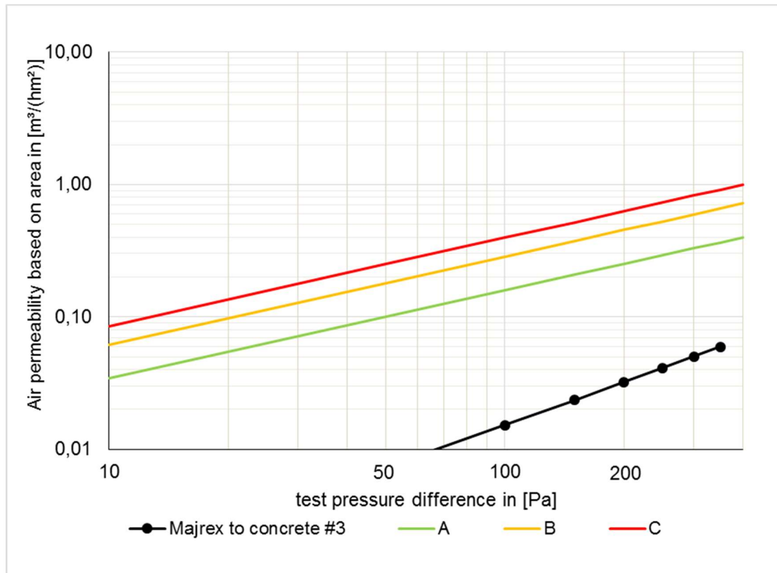
Fig. 17: Series of measurements for the sample "SIGA Majrex to concrete slab #3". The certificate classes A to C according to the PHI are entered in addition.
