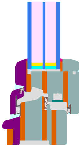
Calculation model
