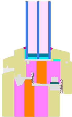
Calculation model
