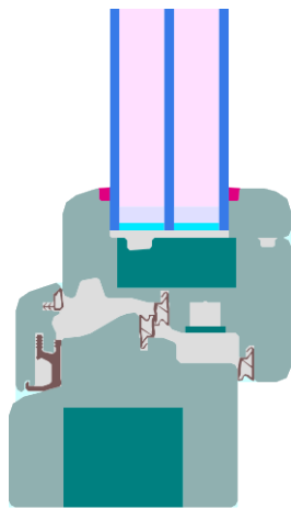
Calculation model
