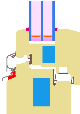
Calculation model
