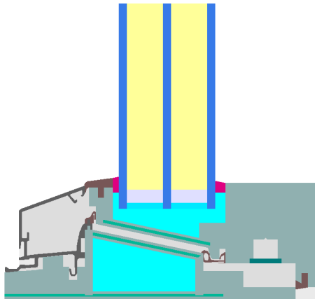
Calculation model
