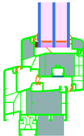
Calculation model
