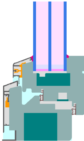
Calculation model
