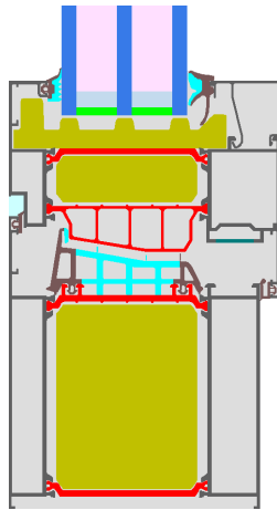
Calculation model
