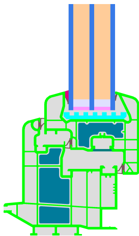
Calculation model
