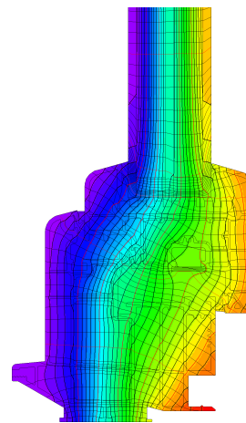
Isothermal
