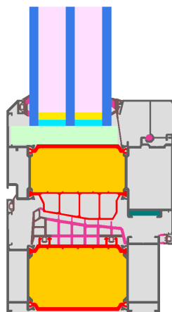
Calculation model
