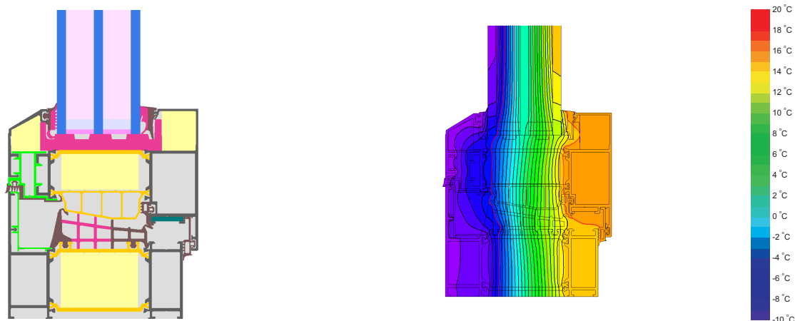
Calculation model
