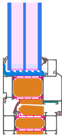
Calculation model
