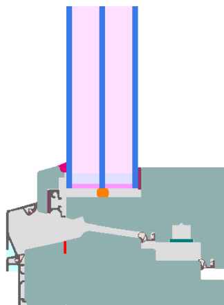
Calculation model
