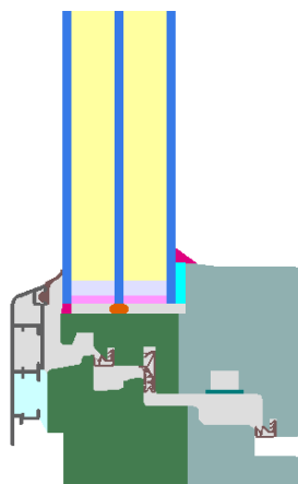
Calculation model
