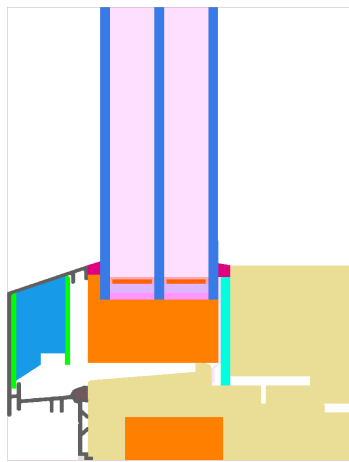
Calculation model
