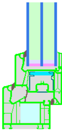
Calculation model
