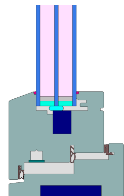
(Outward opening)
