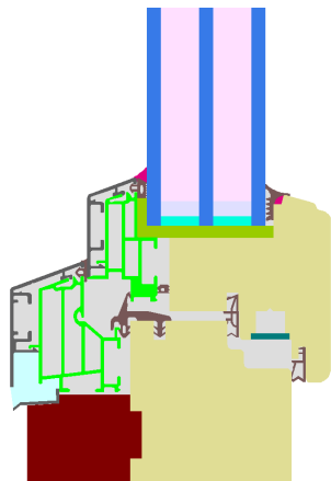
Calculation model
