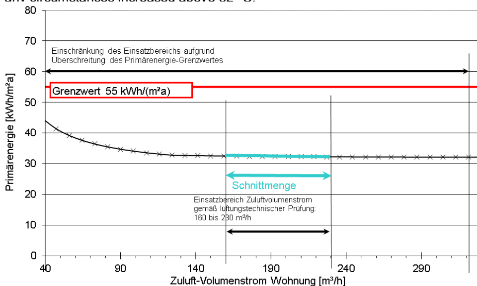
Figure 2: Application range of the unit
