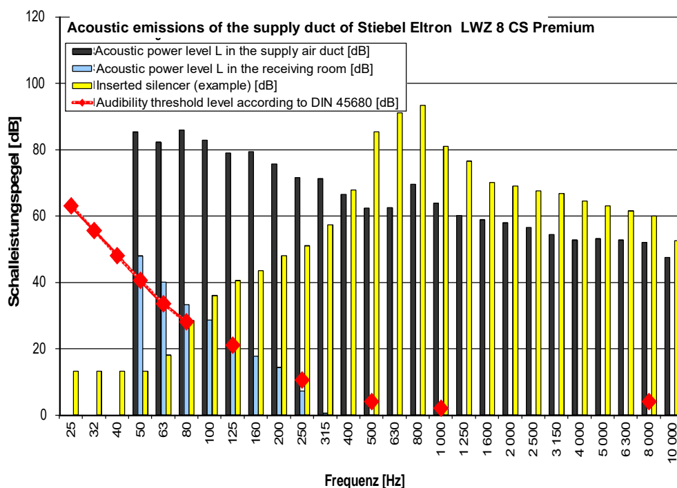
Figure 1: Acoustic emissions of supply duct of the unit [dB]
