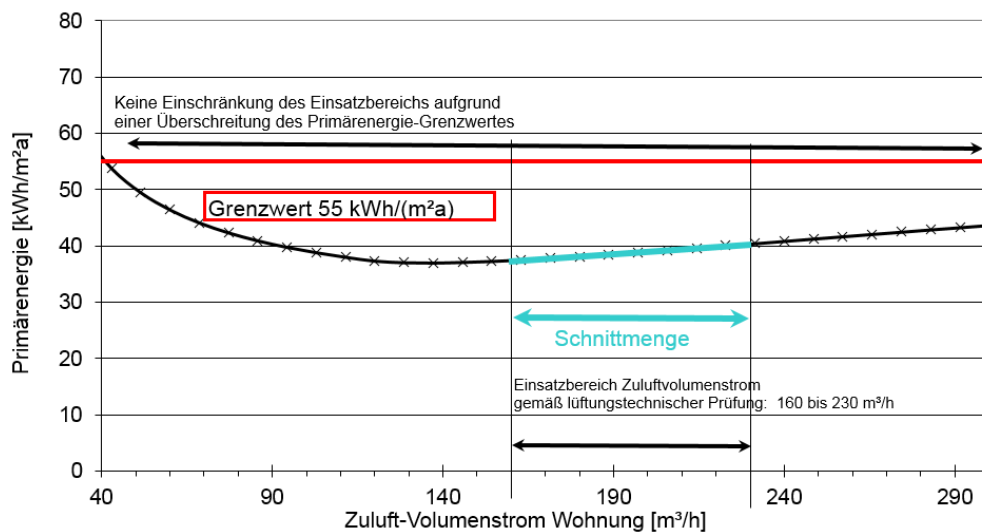
Figure 2: Application range of the unit
