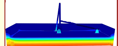
Isothermal map of the Passive House Attic Stairs
