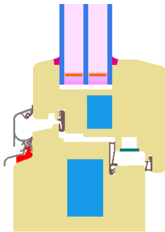
Calculation model
