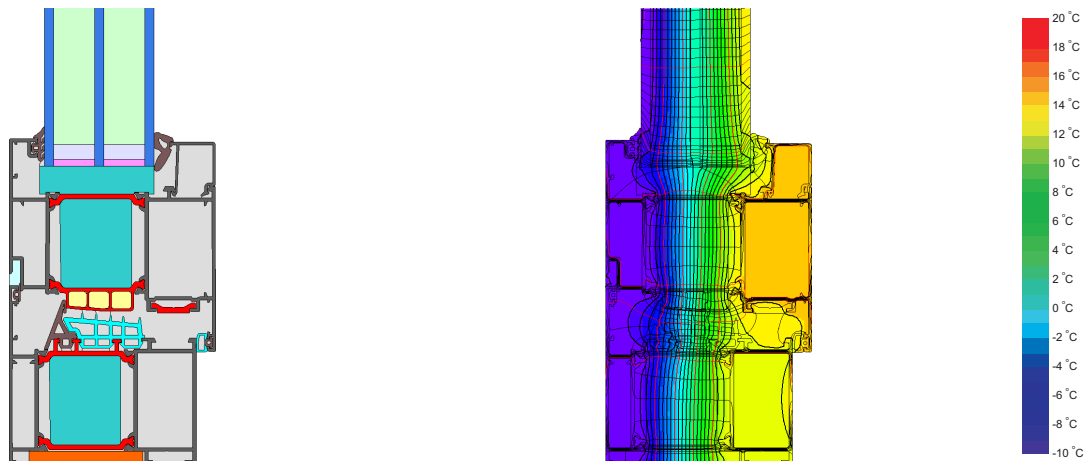
Calculation model
