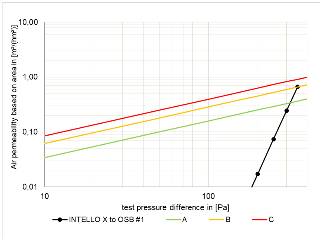
Fig. 9: Series of measurements for the sample "INTELLO X to OSB #1". The Certification Classes A to C according to the PHI are entered in addition.
