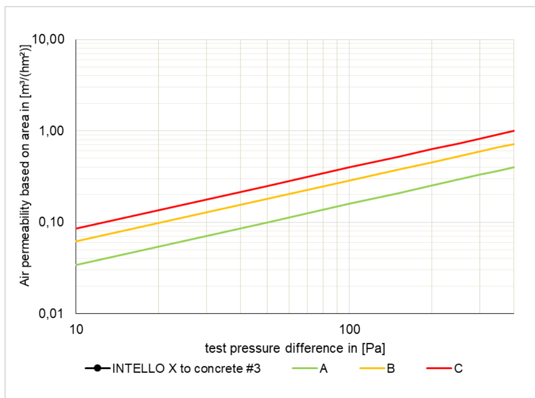
Fig. 15: Series of measurements for the sample "INTELLO X to concrete #3". The Certification Classes A to C according to the PHI are entered in addition.
