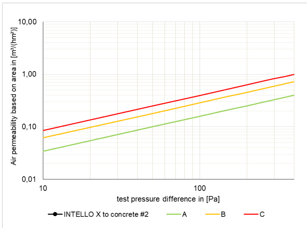
Fig. 14: Series of measurements for the sample "INTELLO X to concrete #2". The Certification Classes A to C according to the PHI are entered in addition.
