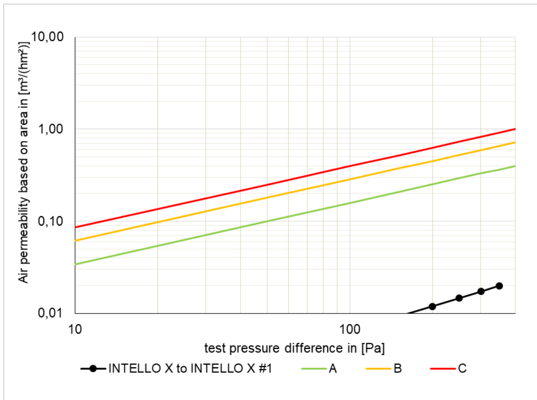
Fig. 6: Series of measurements for the sample "INTELLO X to INTELLO X #1". The Certification Classes A to C according to the PHI are entered in addition.
