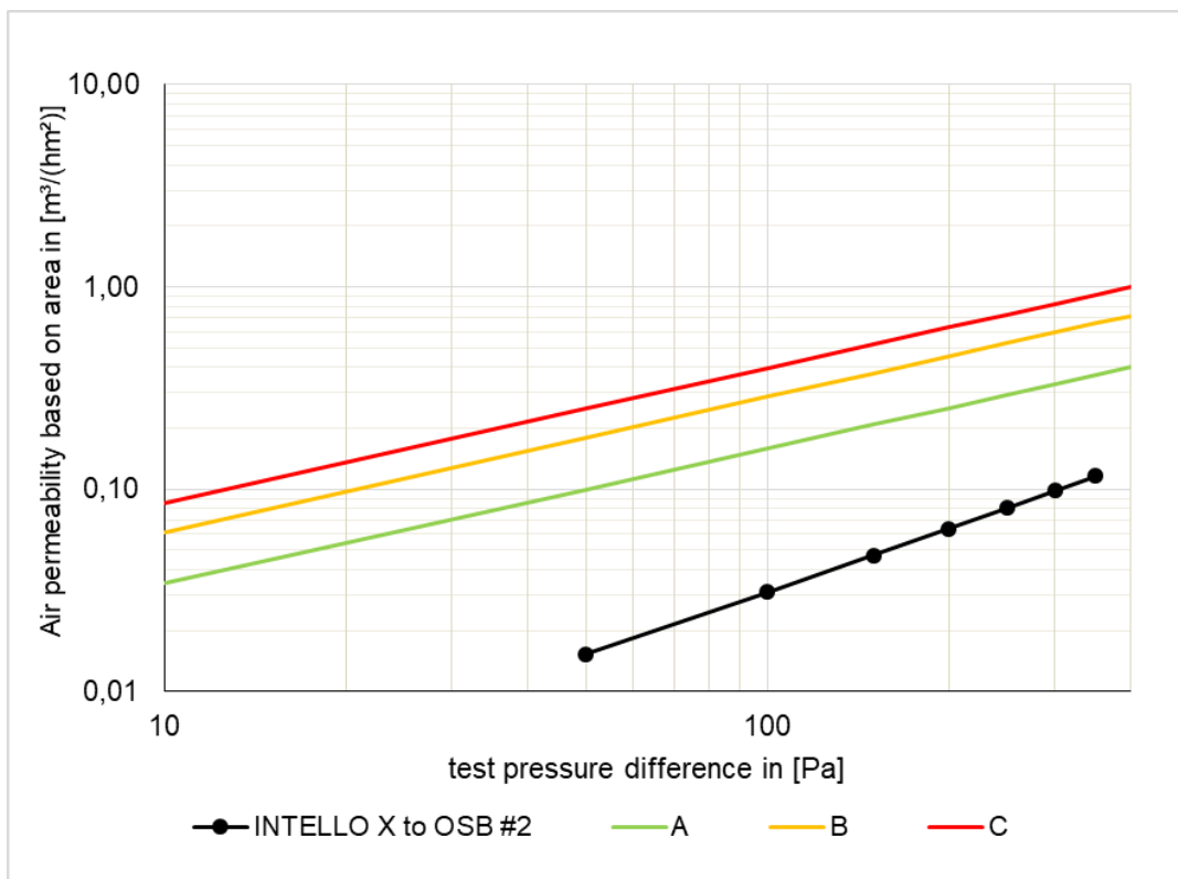
Fig. 10: Series of measurements for the sample "INTELLO X to OSB #2". The Certification Classes A to C according to the PHI are entered in addition.
