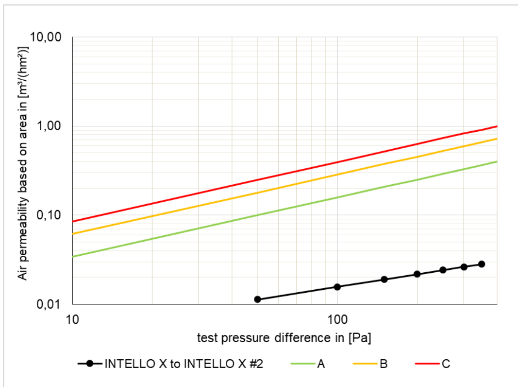
Fig. 7: Series of measurements for the sample "INTELLO X to INTELLO X #2". The Certification Classes A to C according to the PHI are entered in addition.
