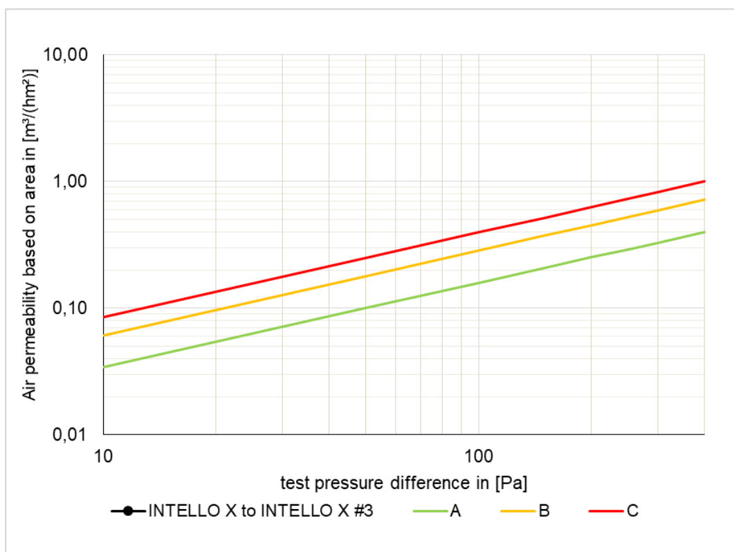
Fig. 8: Series of measurements for the sample "INTELLO X to INTELLO X #3". The Certification Classes A to C according to the PHI are entered in addition.
