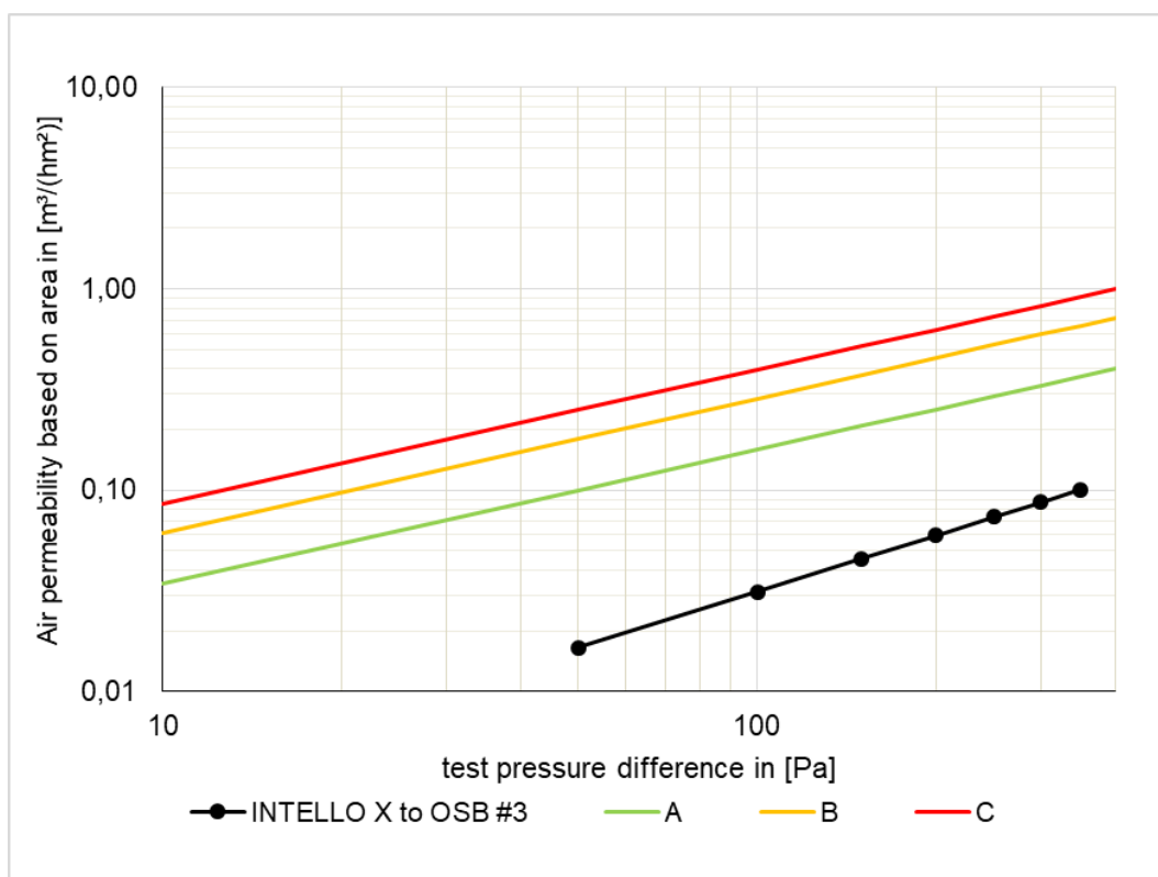
Fig. 11: Series of measurements for the sample "INTELLO X to OSB #3". The Certification Classes A to C according to the PHI are entered in addition.
