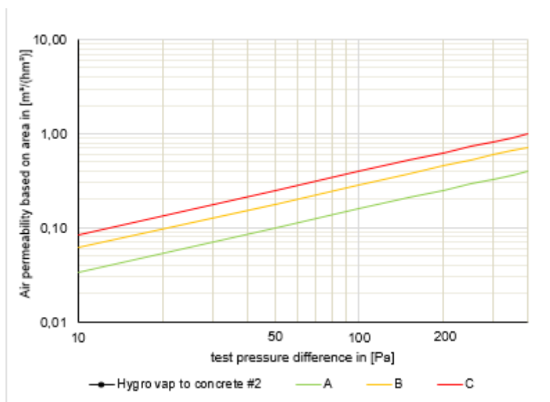
Fig. 14: Series of measurements for the sample "HYGRO'VAP to concrete #2". The Certification Classes A to C according to the PHI are entered in addition.
