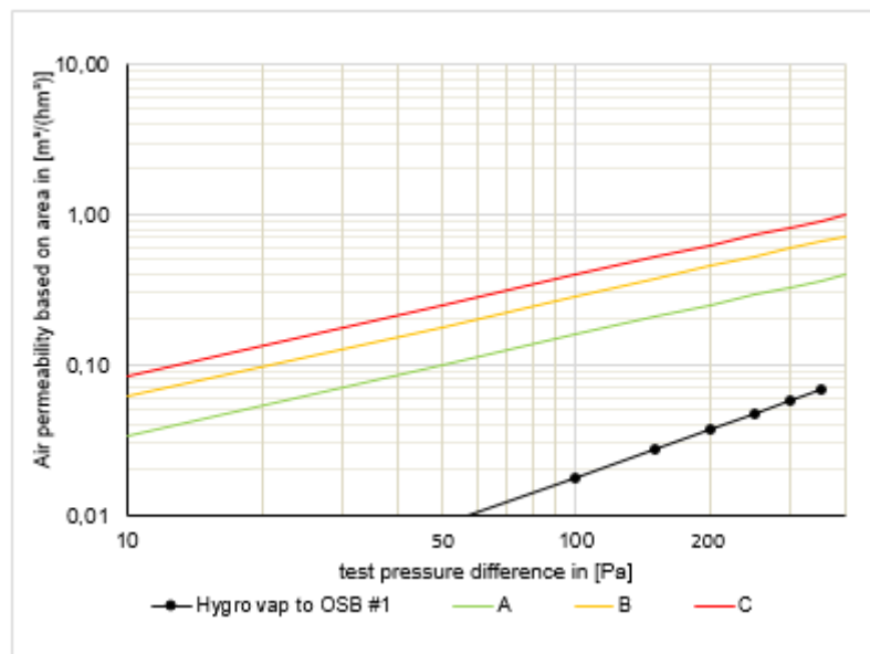
Fig. 9: Series of measurements for the sample "HYGRO'VAP to OSB #1". The Certification Classes A to C according to the PHI are entered in addition.
