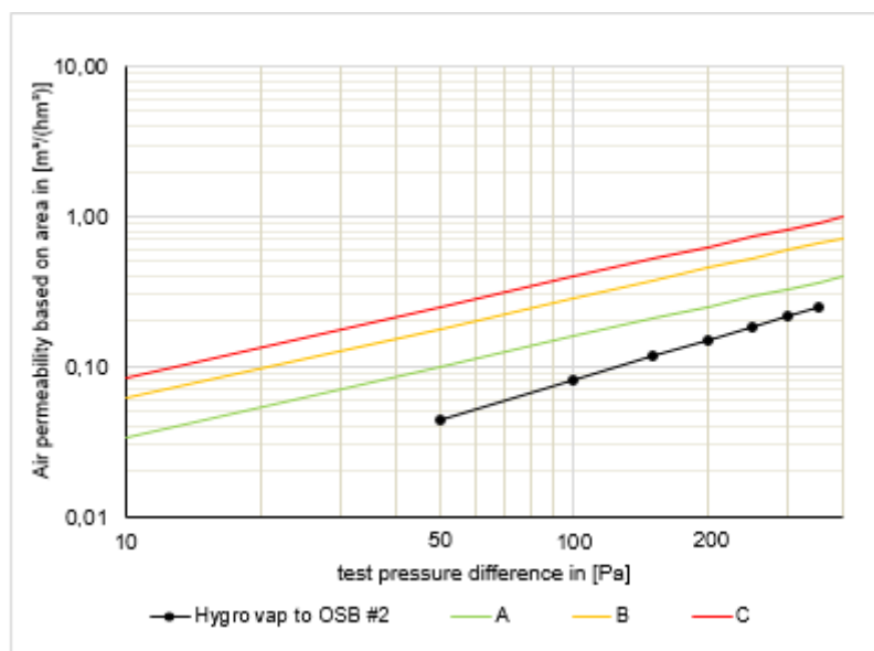
Fig. 10: Series of measurements for the sample "HYGRO'VAP to OSB #2". The Certification Classes A to C according to the PHI are entered in addition.
