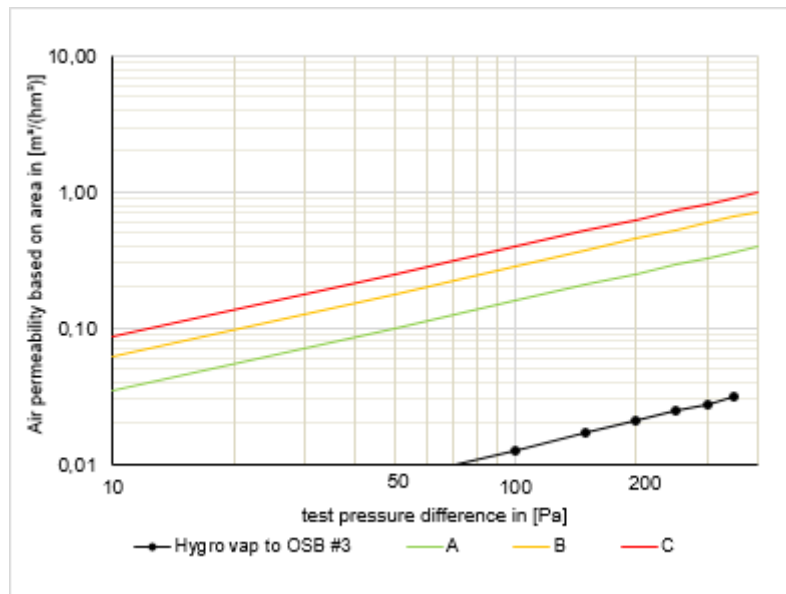
Fig. 11: Series of measurements for the sample "HYGRO'VAP to OSB #3". The Certification Classes A to C according to the PHI are entered in addition.
