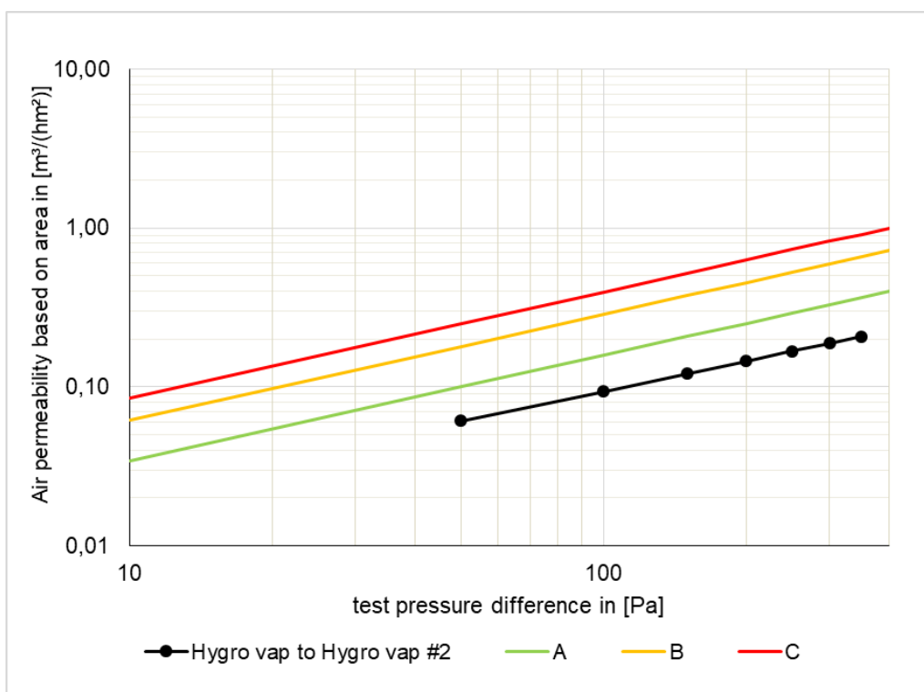
Fig. 7: Series of measurements for the sample "HYGRO'VAP to HYGRO'VAP #2". The Certification Classes A to C according to the PHI are entered in addition.
