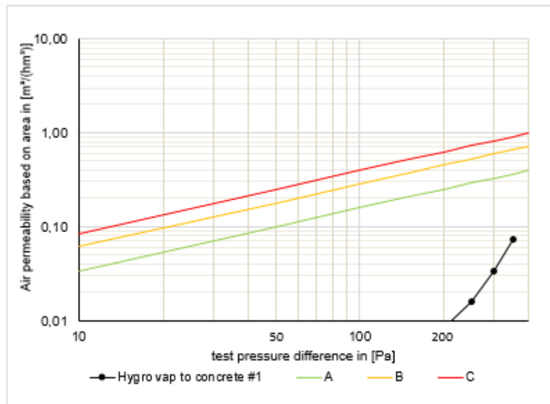
Fig. 13: Series of measurements for the sample "HYGRO'VAP to concrete #1". The Certification Classes A to C according to the PHI are entered in addition.
