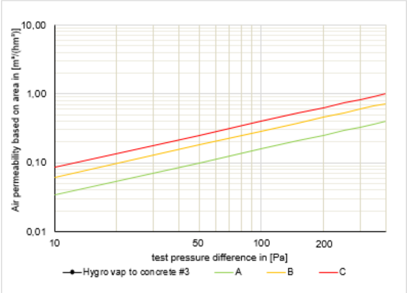
Fig. 15: Series of measurements for the sample "HYGRO'VAP to concrete #3". The Certification Classes A to C according to the PHI are entered in addition.
