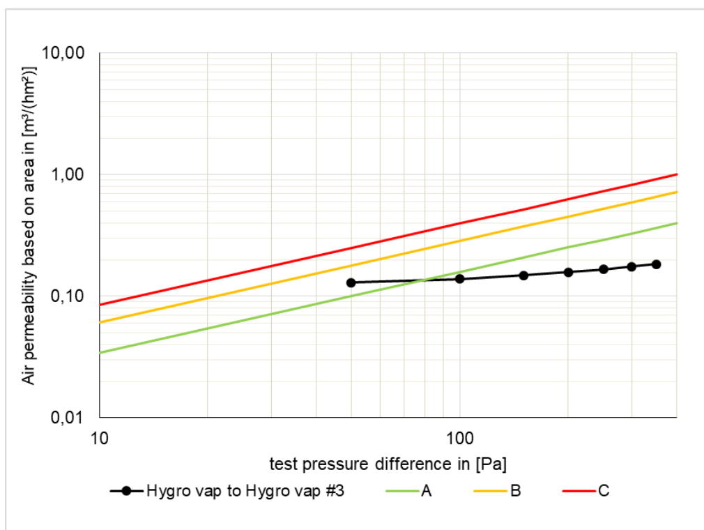
Fig. 8: Series of measurements for the sample "HYGRO'VAP to HYGRO'VAP #3". The Certification Classes A to C according to the PHI are entered in addition.
