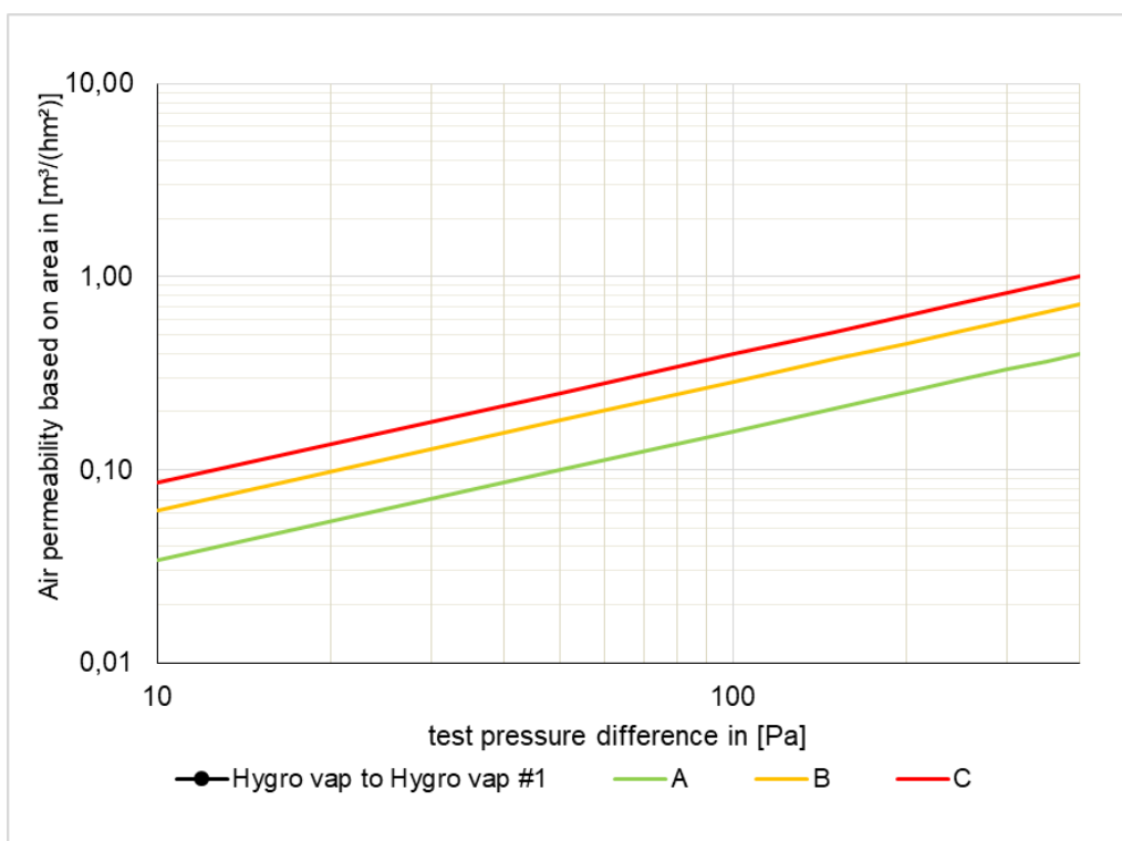
Fig. 6: Series of measurements for the sample "HYGRO'VAP to HYGRO'VAP #1". The Certification Classes A to C according to the PHI are entered in addition.
