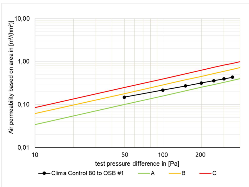
Fig. 9: Series of measurements for the sample "Clima Control 80 to OSB #1". The Certification Classes A to C according to the PHI are entered in addition.
