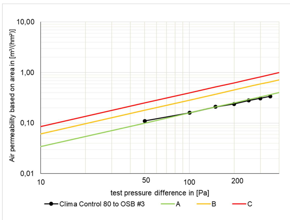
Fig. 11: Series of measurements for the sample "Clima Control 80 to OSB #3". The Certification Classes A to C according to the PHI are entered in addition.
