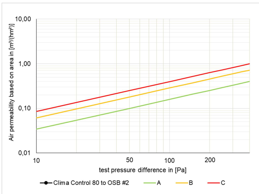
Fig. 10: Series of measurements for the sample "Clima Control 80 to OSB #2". The Certification Classes A to C according to the PHI are entered in addition.
