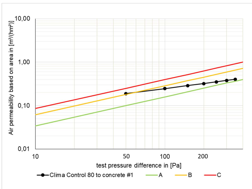
Fig. 12: Series of measurements for the sample "Clima Control 80 to concrete #1". The Certification Classes A to C according to the PHI are entered in addition.
