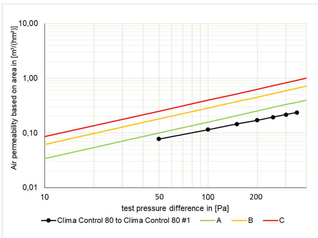
Fig. 6: Series of measurements for the sample "Clima Control 80 to Clima Control 80 #1". The Certification Classes A to C according to the PHI are entered in addition.
