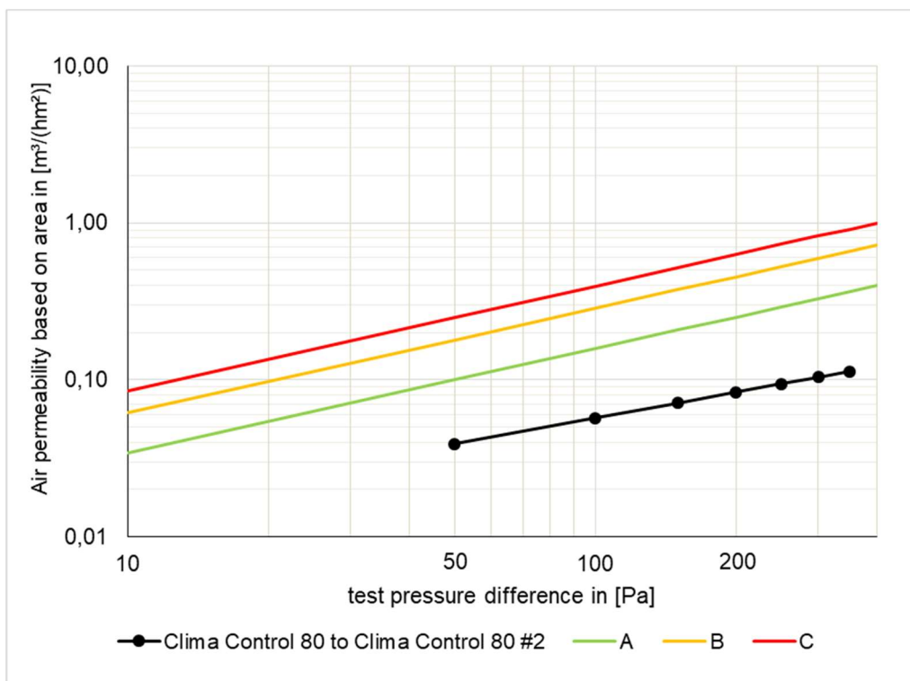
Fig. 7: Series of measurements for the sample "Clima Control 80 to Clima Control 80 #2". The Certification Classes A to C according to the PHI are entered in addition.
