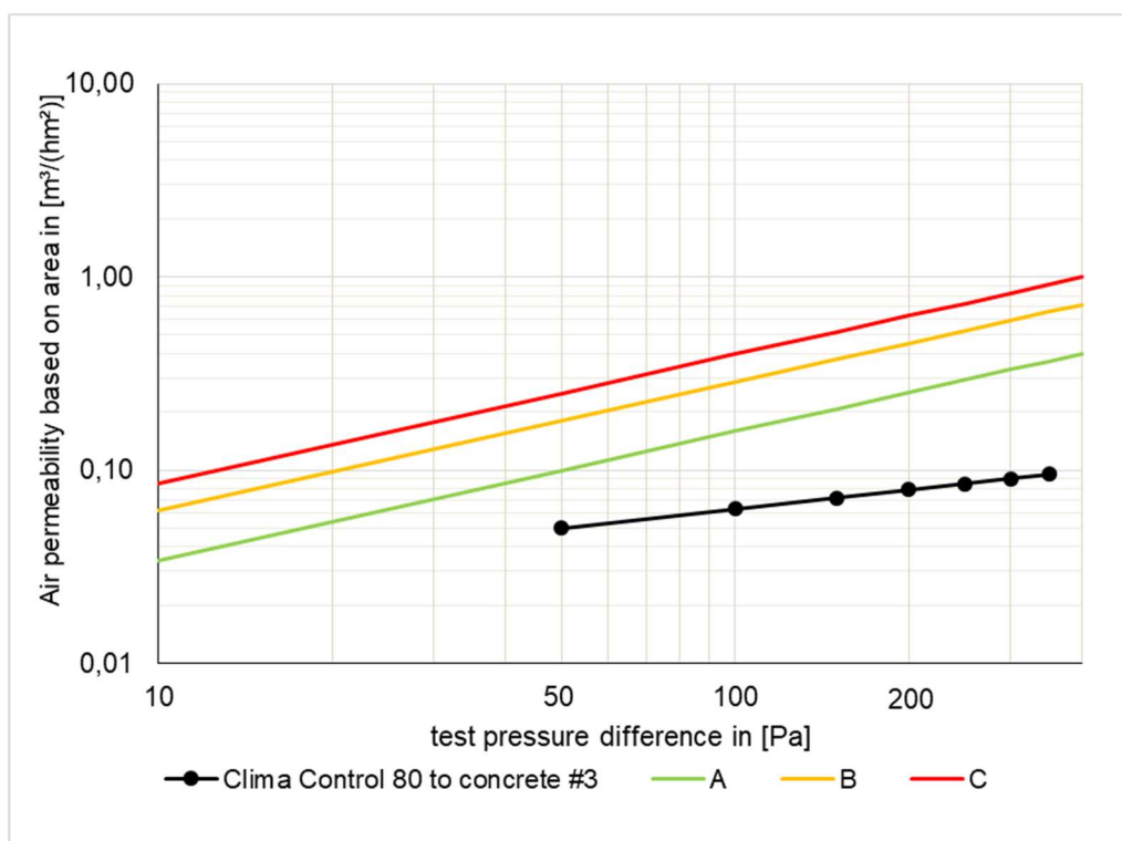
Fig. 14: Series of measurements for the sample "Clima Control 80 to concrete #3". The Certification Classes A to C according to the PHI are entered in addition.
