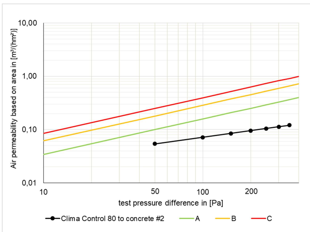
Fig. 13: Series of measurements for the sample "Clima Control 80 to concrete #2". The Certification Classes A to C according to the PHI are entered in addition.
