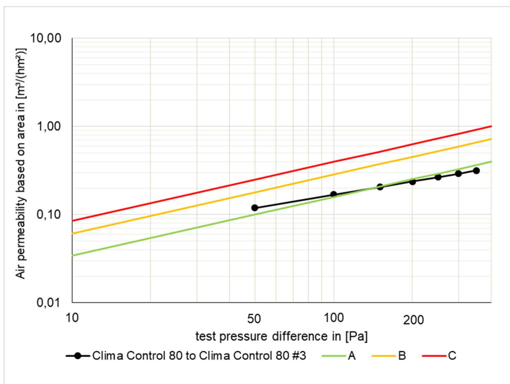
Fig. 8: Series of measurements for the sample "Clima Control 80 to Clima Control 80 #3". The Certification Classes A to C according to the PHI are entered in addition.
