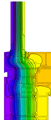
Isothermal
