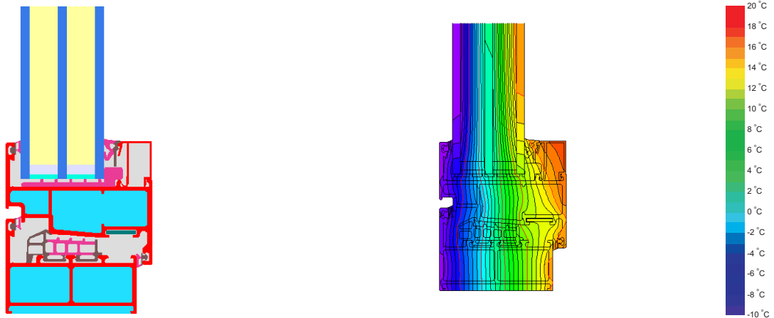
Calculation model
