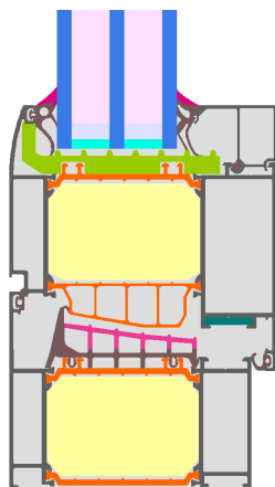
Calculation model
