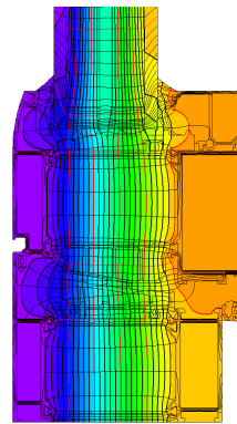
Isothermal
