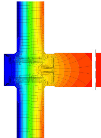
Isothermal
