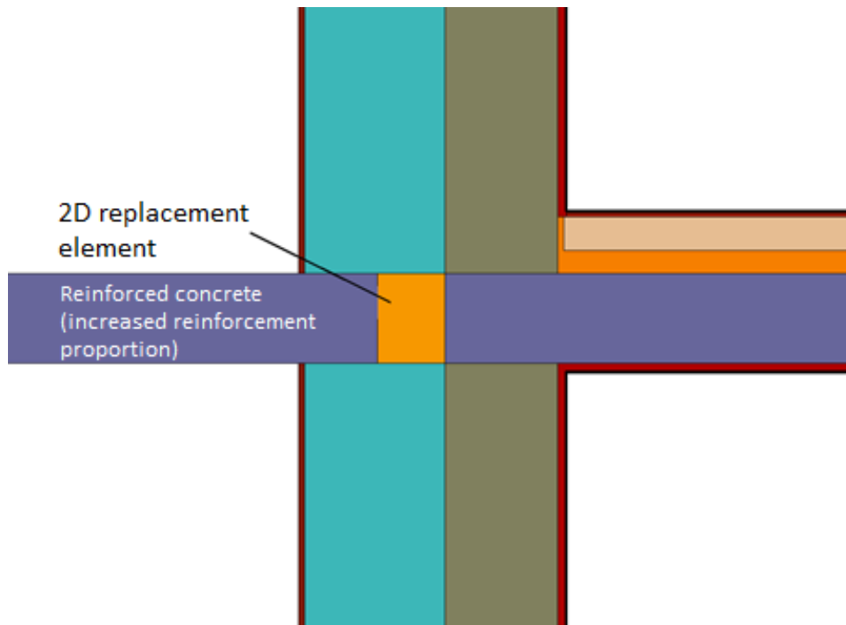
Figure 3: 2D replacement model – taking the reinforcing bars into account by increasing the thermal conductivity of the reinforced concrete in the area of the connection element
