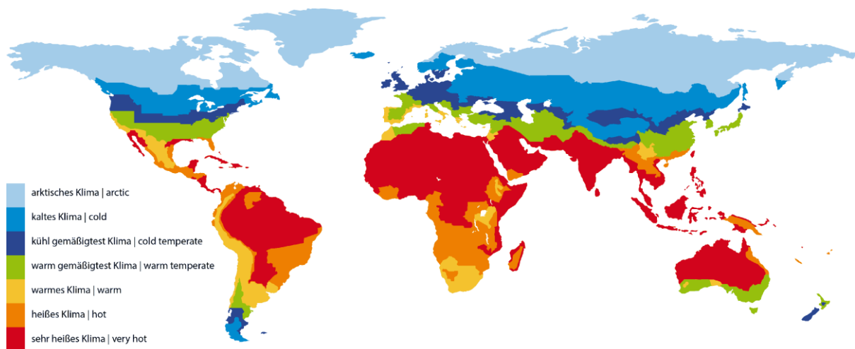
Figure 1: Climate zones
