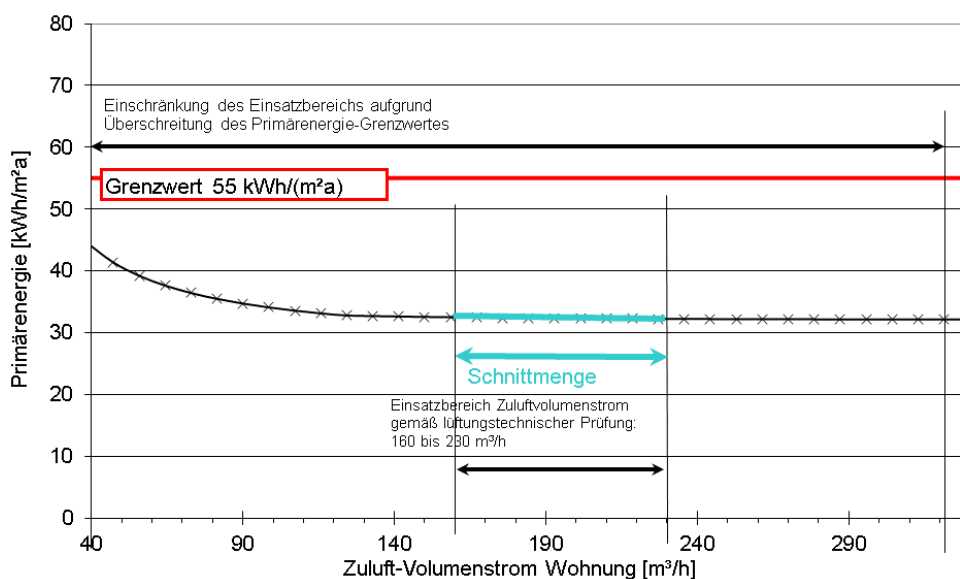
Figure 2: Application range of the unit Stiebel Eltron LWZ 504
