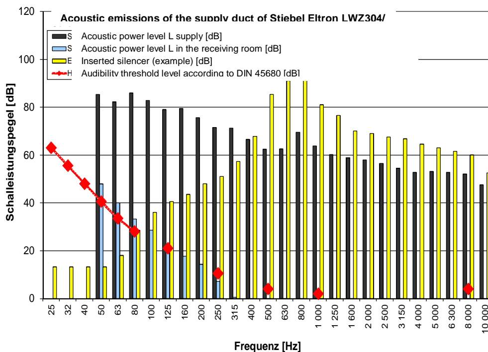
Figure 1: Acoustic emissions of supply duct of the unit Stiebel Eltron LWZ 504 [dB]
