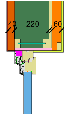
Ext insulation a. finish. s. (EIFS) threshold ceiling (operable)
