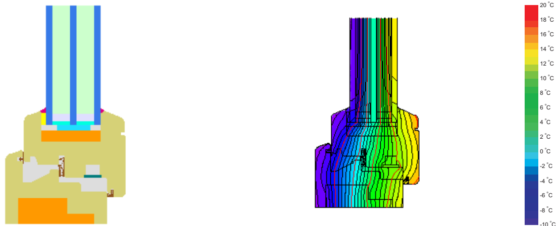
Calculation model
