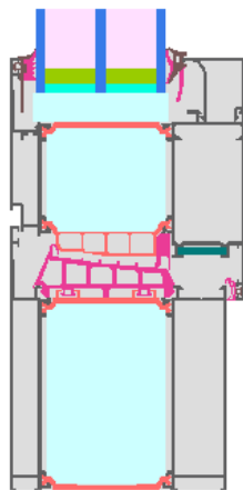
Calculation model
