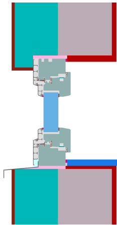
Exterior insulation and finishing system
