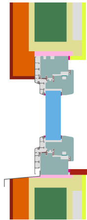
Lightweight timber (operable)
