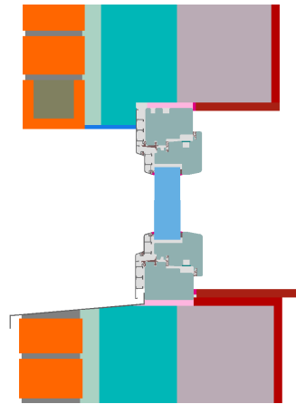
Cavity wall
