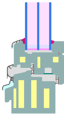
Calculation model
